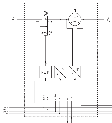
MASTER MODULE SCHEME
