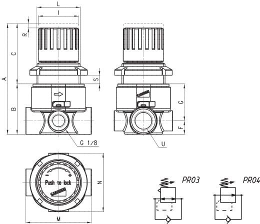
PR03 = regulator with relieving and by-pass valve
